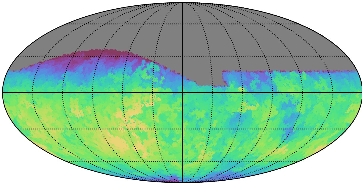
baseline_v2.0_10yrs All sky g band: Max fiveSigmaDepth
