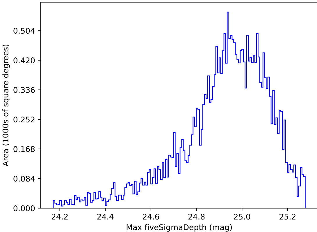
baseline_v2.0_10yrs All sky g band: Max fiveSigmaDepth
