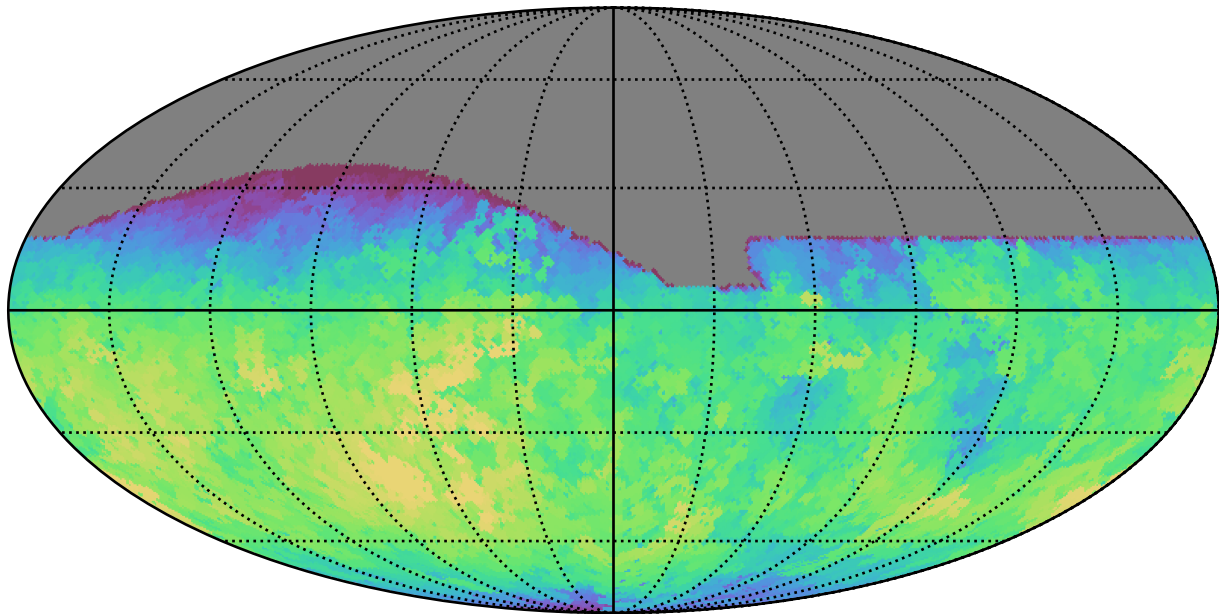
baseline_v2.0_10yrs All sky all bands: Max fiveSigmaDepth
