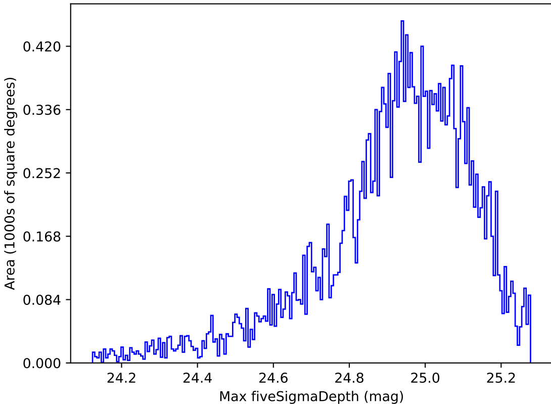
baseline_v2.0_10yrs All sky all bands: Max fiveSigmaDepth
