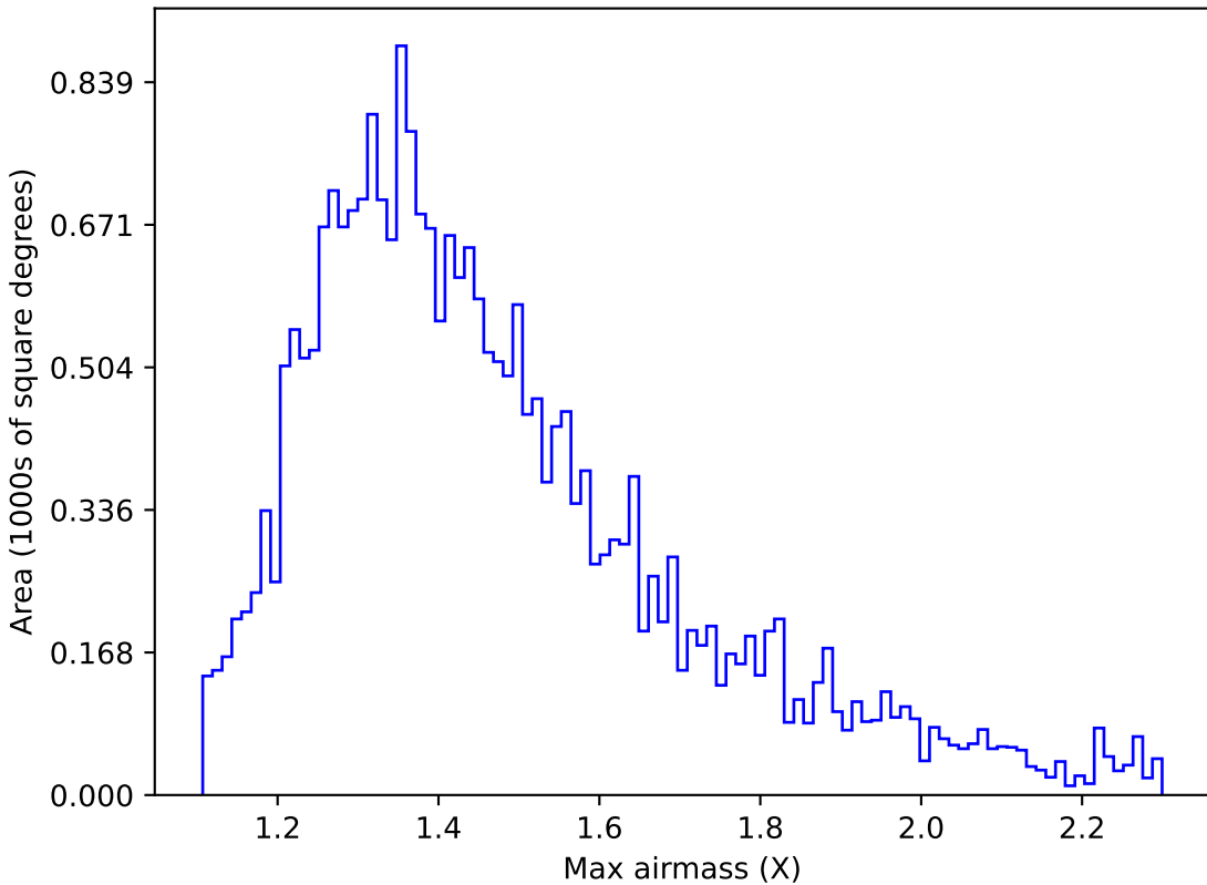
baseline_v2.0_10yrs Yr 1 z band: Max airmass
