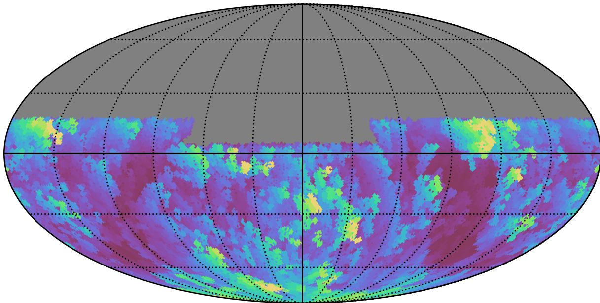
baseline_v2.0_10yrs Yr 1 y band: Max airmass
