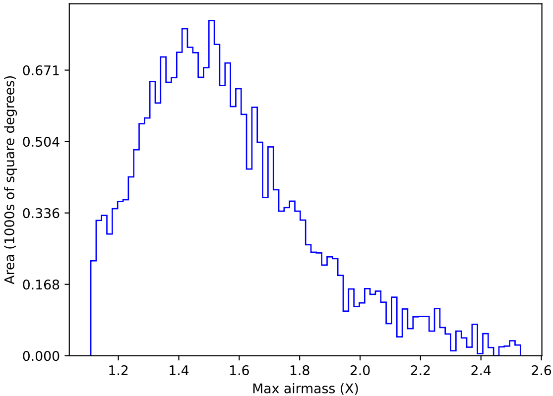
baseline_v2.0_10yrs Yr 1 y band: Max airmass
