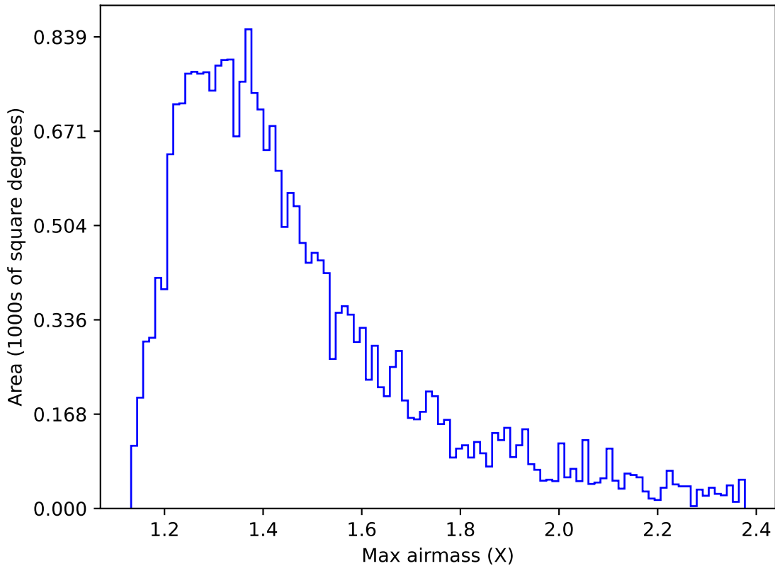
baseline_v2.0_10yrs Yr 1 r band: Max airmass
