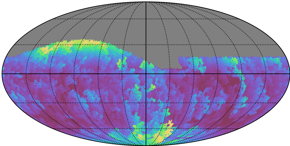
baseline_v2.0_10yrs Yr 1 i band: Max airmass
