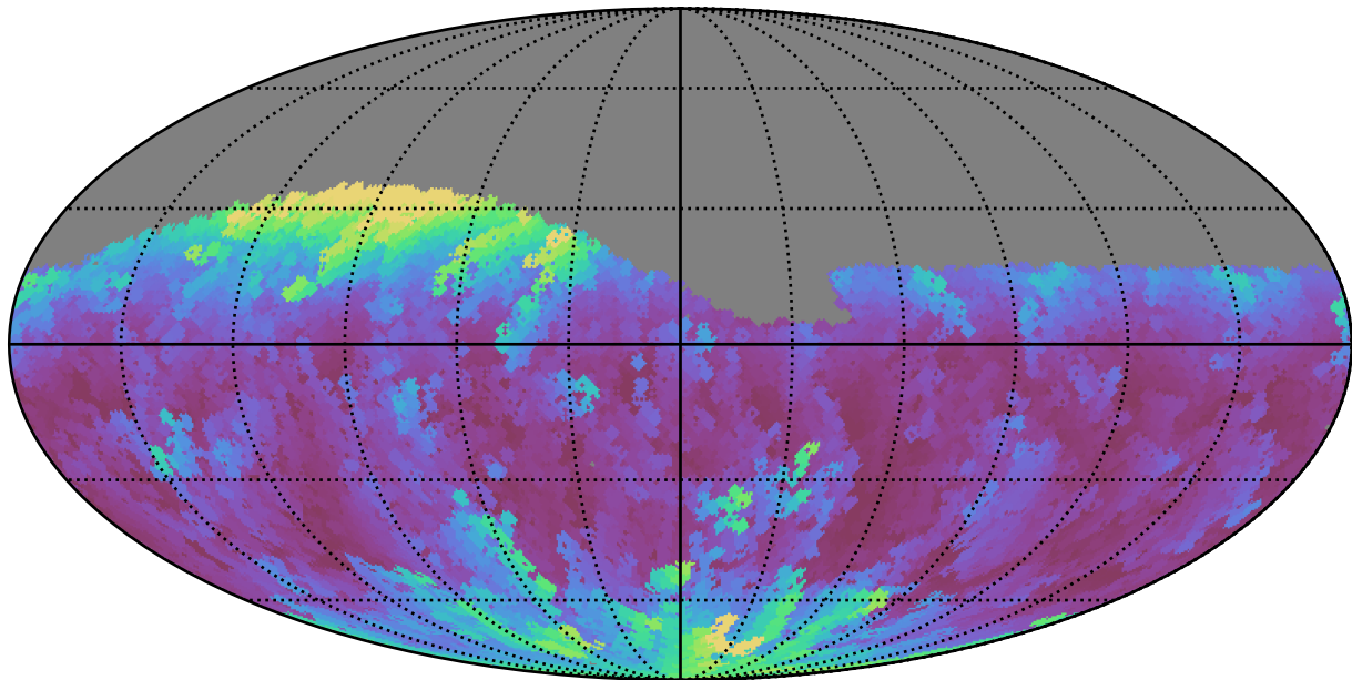
baseline_v2.0_10yrs Yr 1 g band: Max airmass
