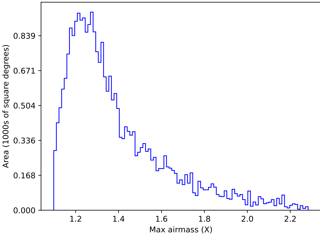
baseline_v2.0_10yrs Yr 1 g band: Max airmass
