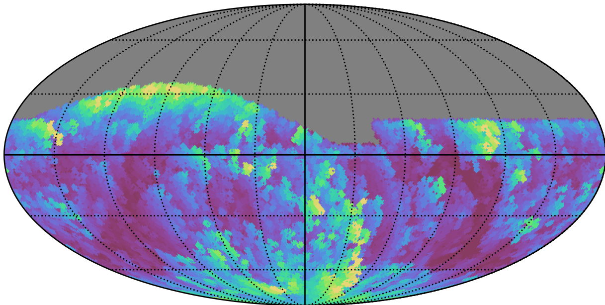
baseline_v2.0_10yrs Yr 1 all bands: Max airmass
