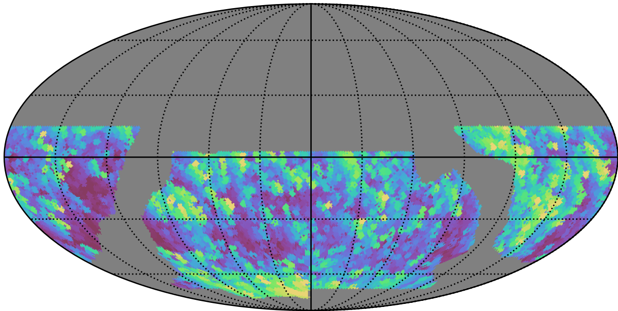
baseline_v2.0_10yrs WFD z band: Max airmass
