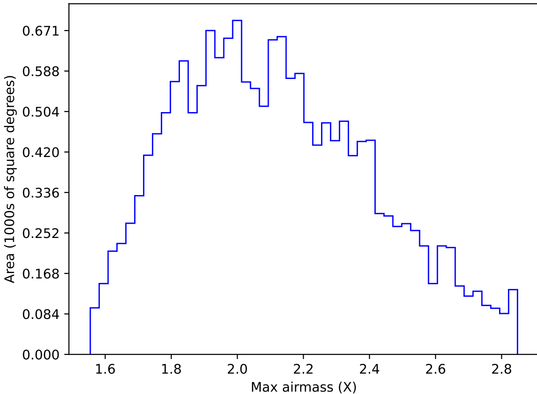
baseline_v2.0_10yrs WFD z band: Max airmass
