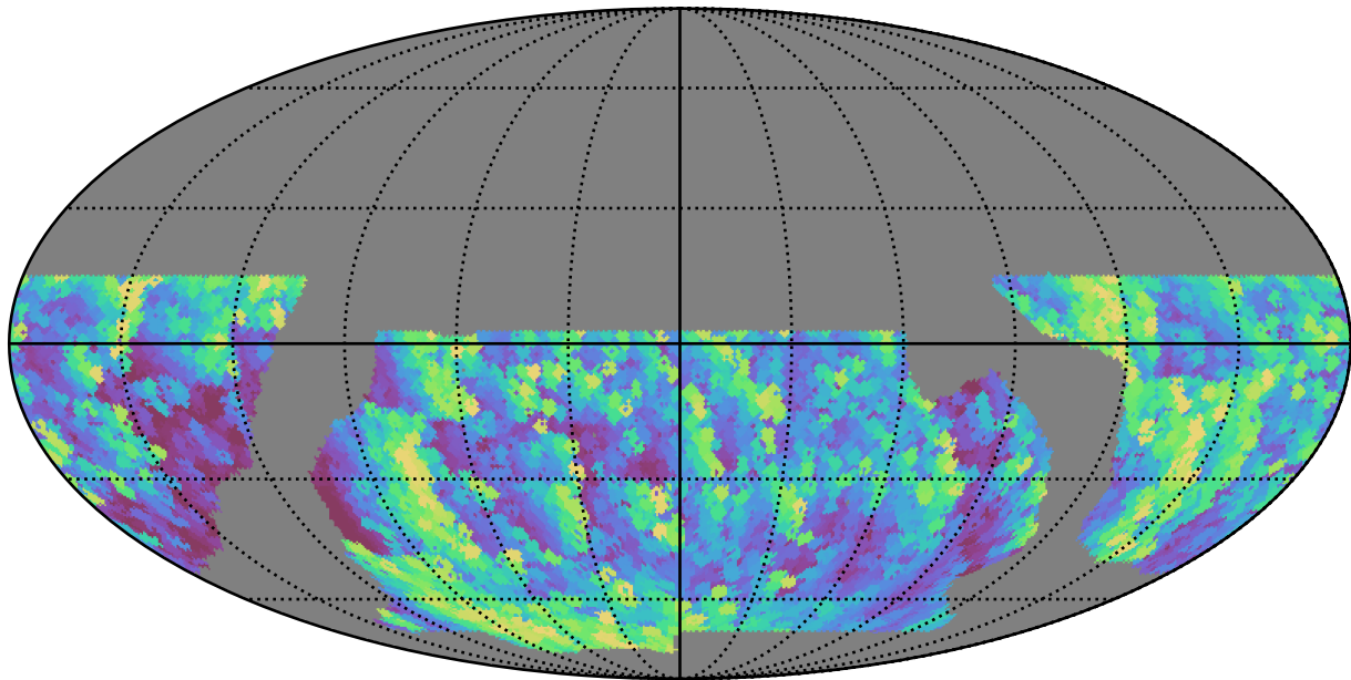
baseline_v2.0_10yrs WFD y band: Max airmass
