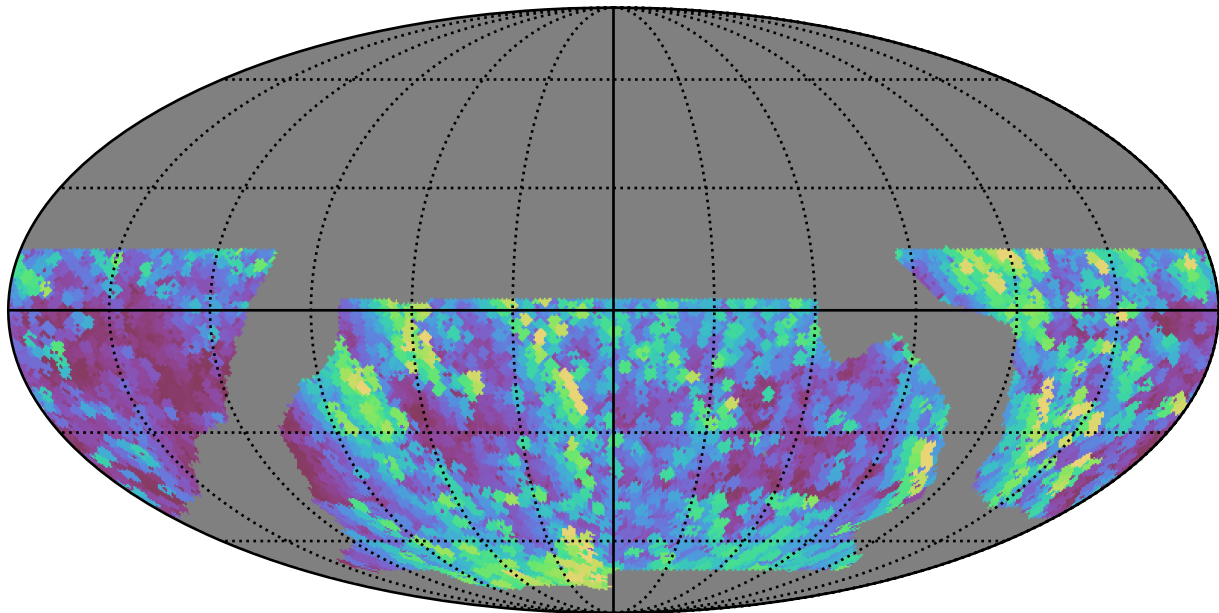
baseline_v2.0_10yrs WFD r band: Max airmass
