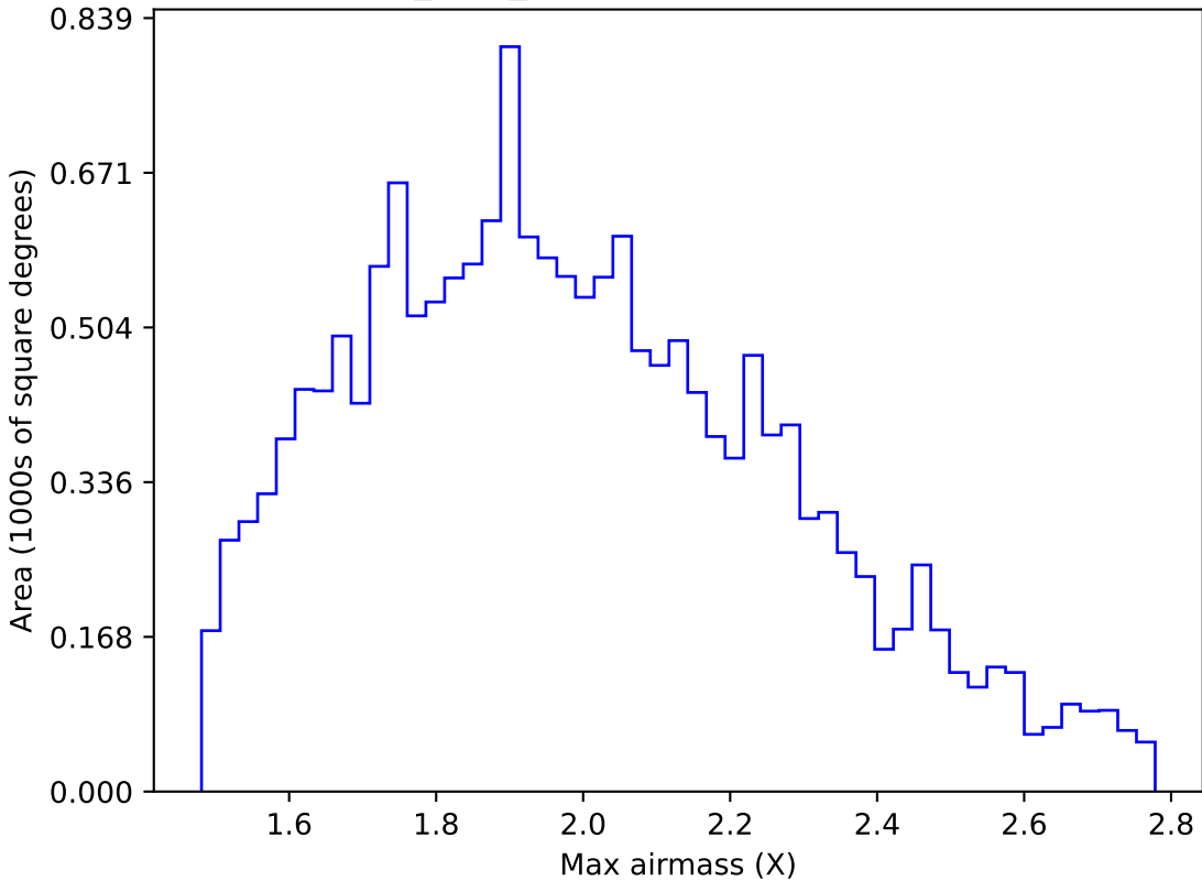
baseline_v2.0_10yrs WFD r band: Max airmass
