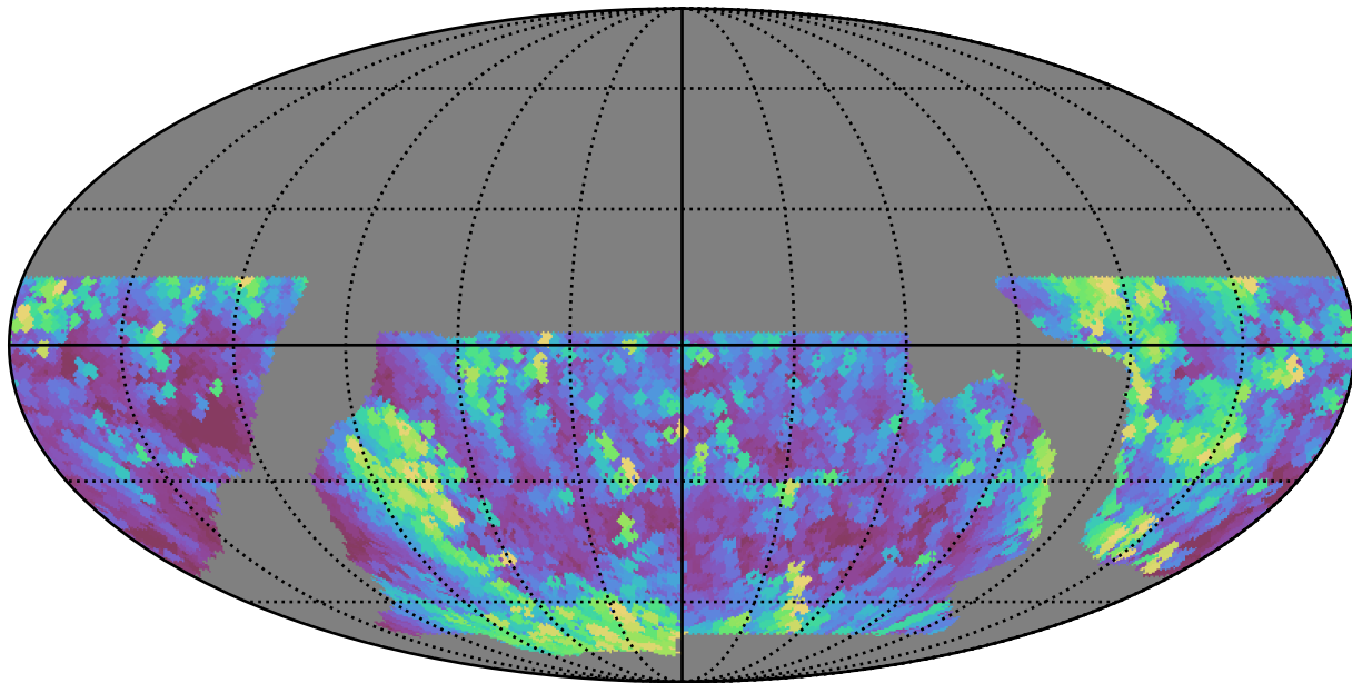
baseline_v2.0_10yrs WFD i band: Max airmass
