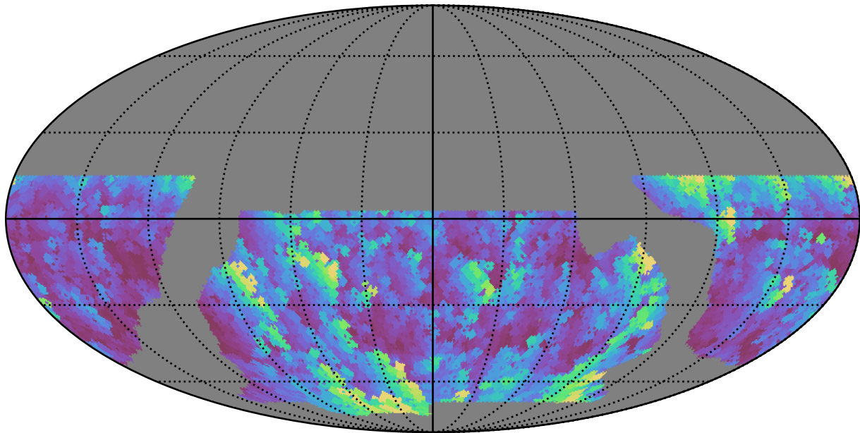
baseline_v2.0_10yrs WFD g band: Max airmass
