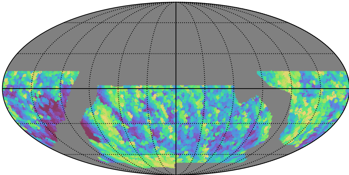
baseline_v2.0_10yrs WFD all bands: Max airmass
