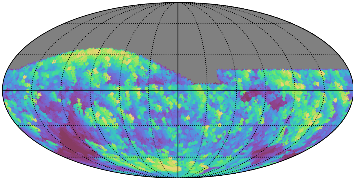
baseline_v2.0_10yrs All sky z band: Max airmass
