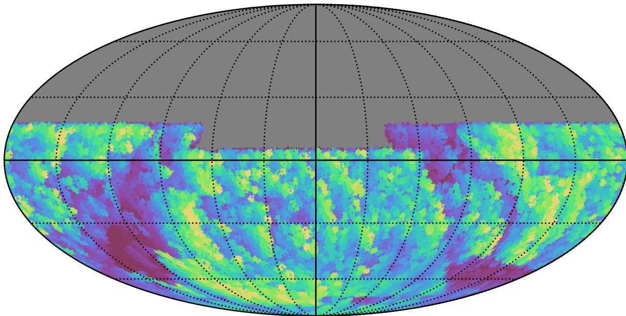
baseline_v2.0_10yrs All sky y band: Max airmass
