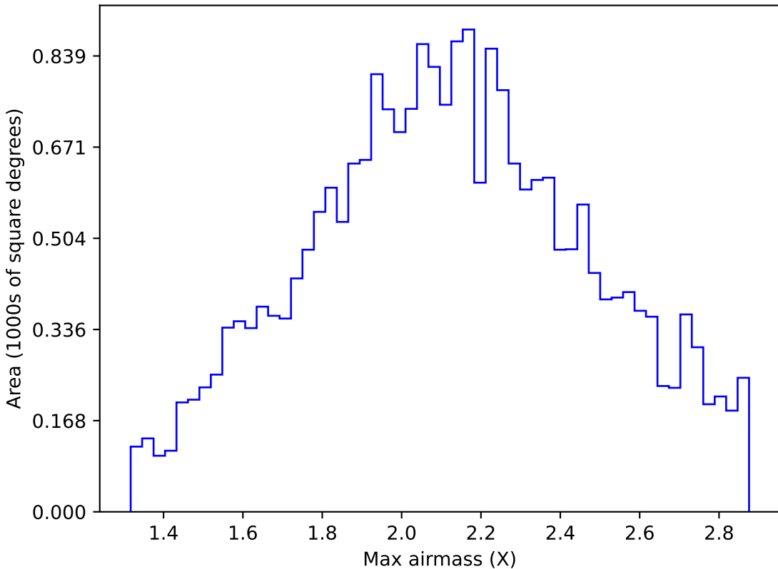
baseline_v2.0_10yrs All sky y band: Max airmass
