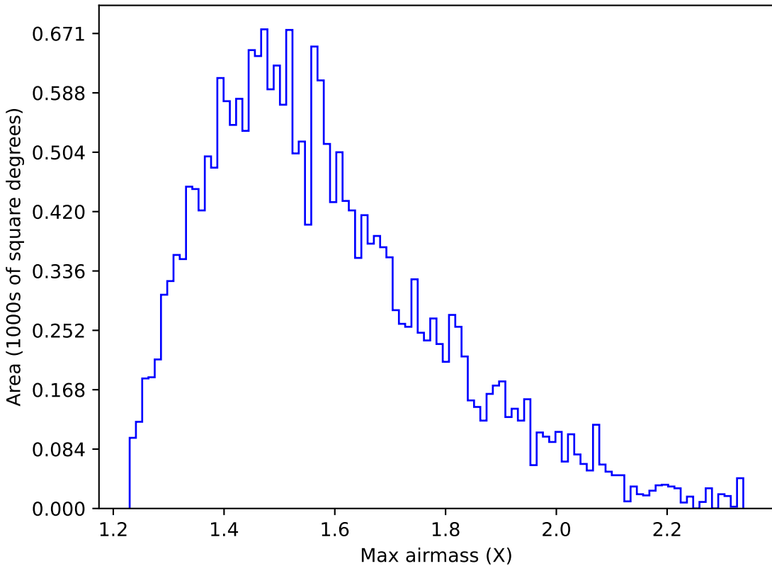
baseline_v2.0_10yrs All sky u band: Max airmass
