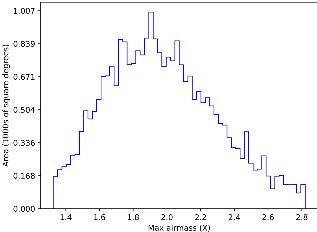
baseline_v2.0_10yrs All sky r band: Max airmass
