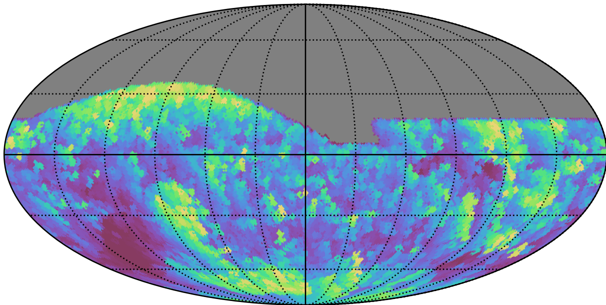
baseline_v2.0_10yrs All sky i band: Max airmass
