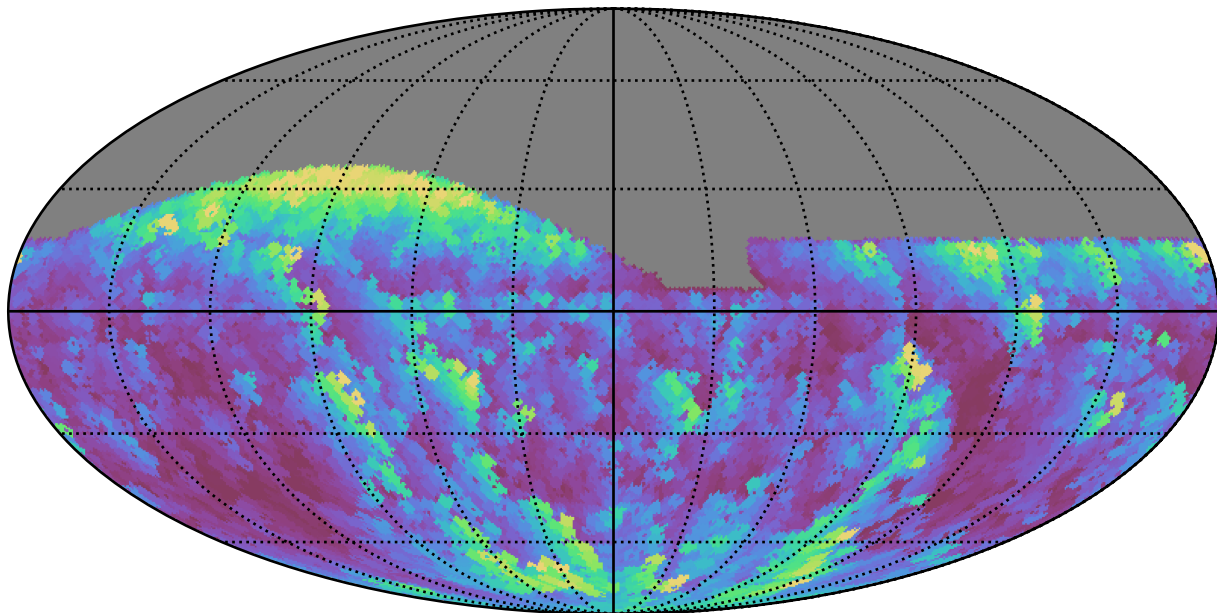
baseline_v2.0_10yrs All sky g band: Max airmass
