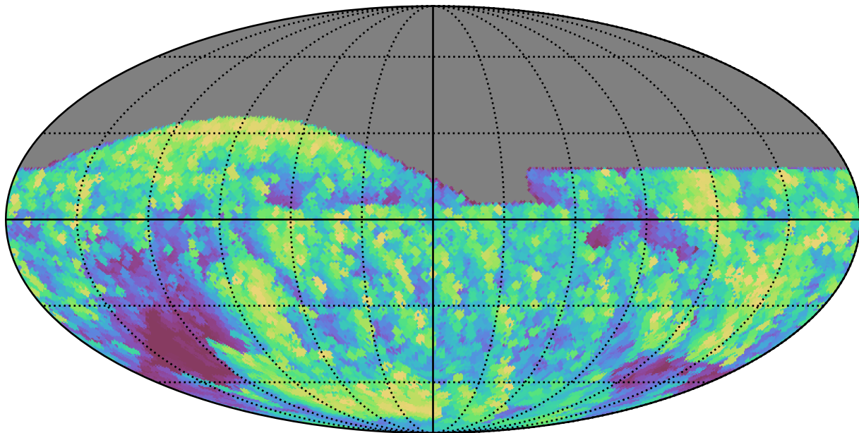
baseline_v2.0_10yrs All sky all bands: Max airmass
