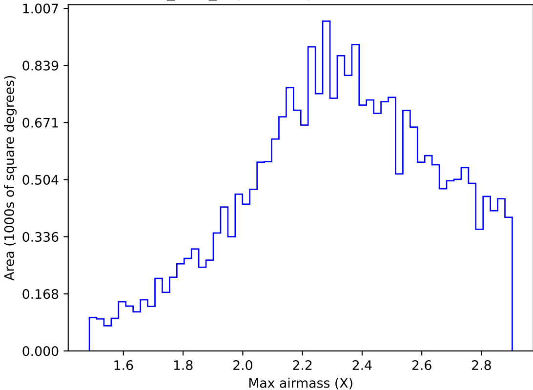
baseline_v2.0_10yrs All sky all bands: Max airmass
