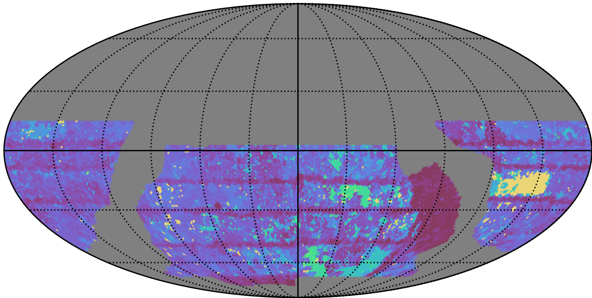
baseline_v2.0_10yrs WFD z band: Max Inter-Night Gap
