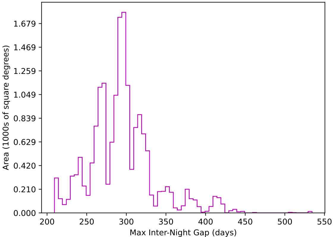
baseline_v2.0_10yrs WFD z band: Max Inter-Night Gap
