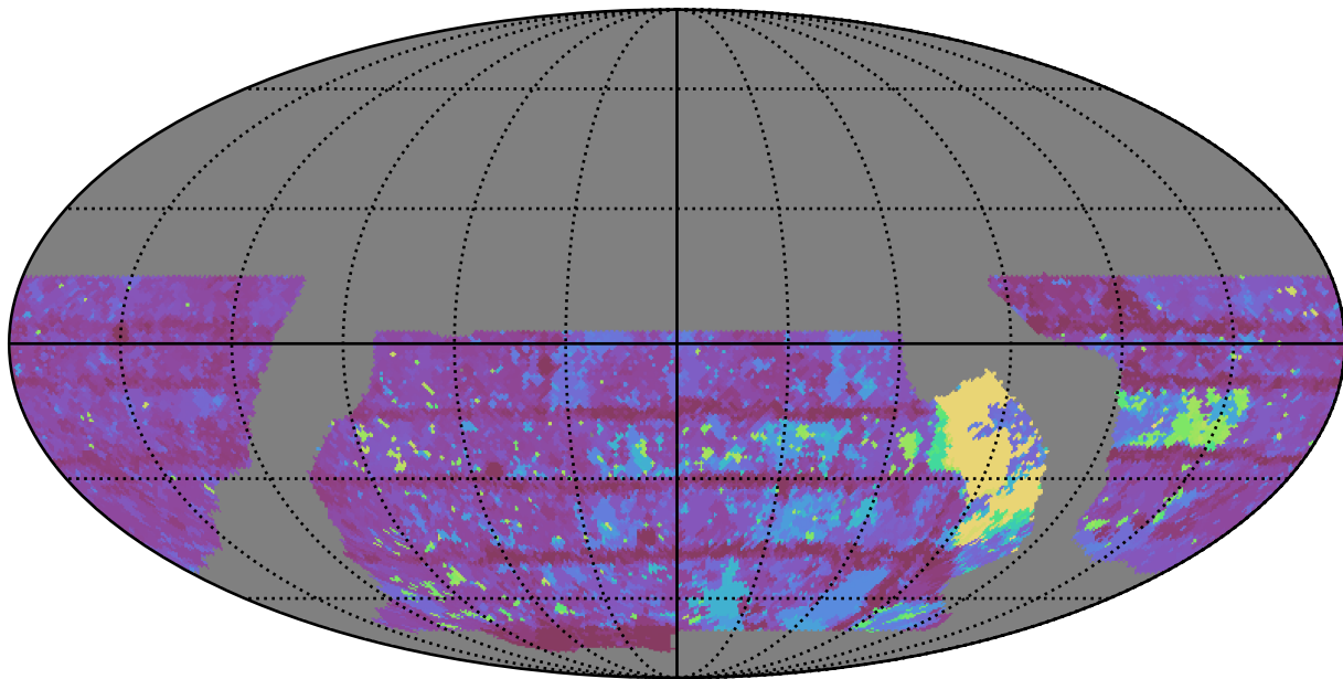
baseline_v2.0_10yrs WFD y band: Max Inter-Night Gap
