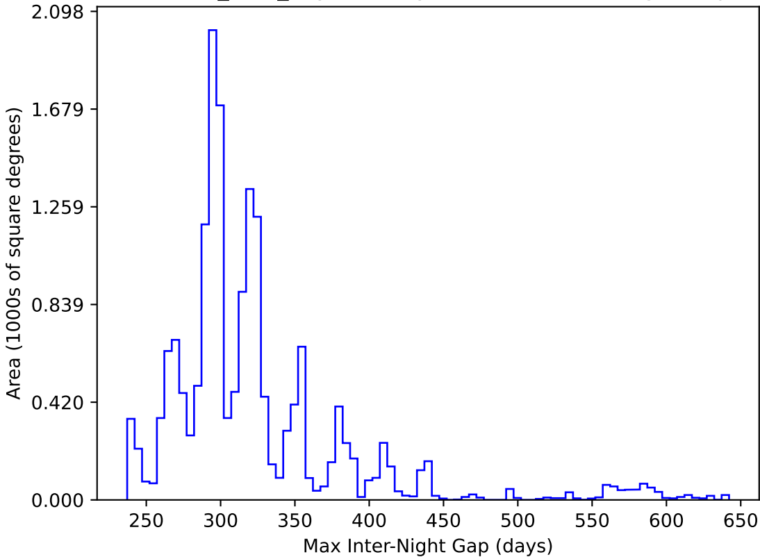
baseline_v2.0_10yrs WFD y band: Max Inter-Night Gap
