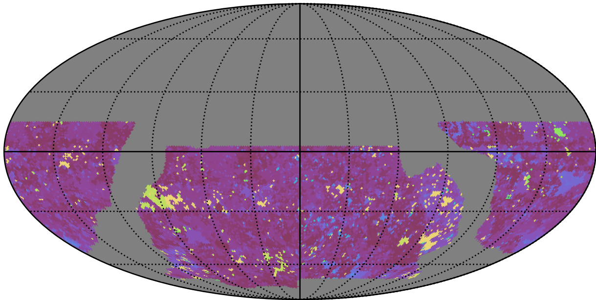
baseline_v2.0_10yrs WFD u band: Max Inter-Night Gap
