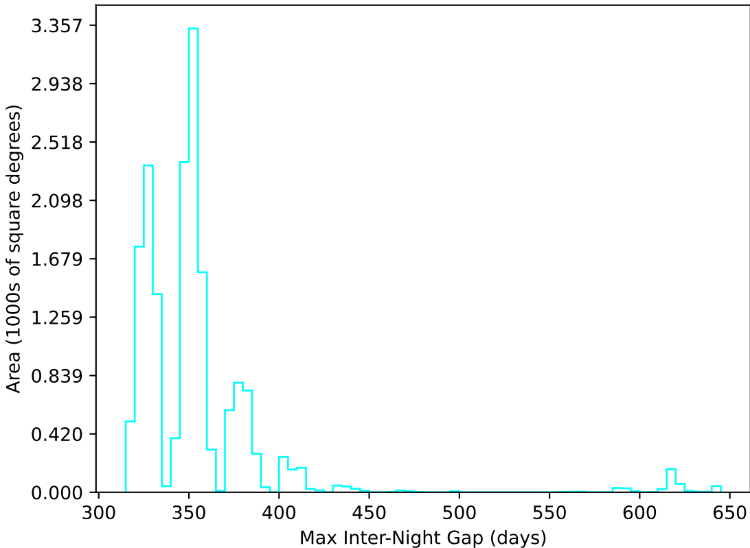
baseline_v2.0_10yrs WFD u band: Max Inter-Night Gap
