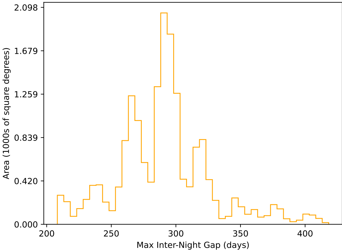
baseline_v2.0_10yrs WFD r band: Max Inter-Night Gap
