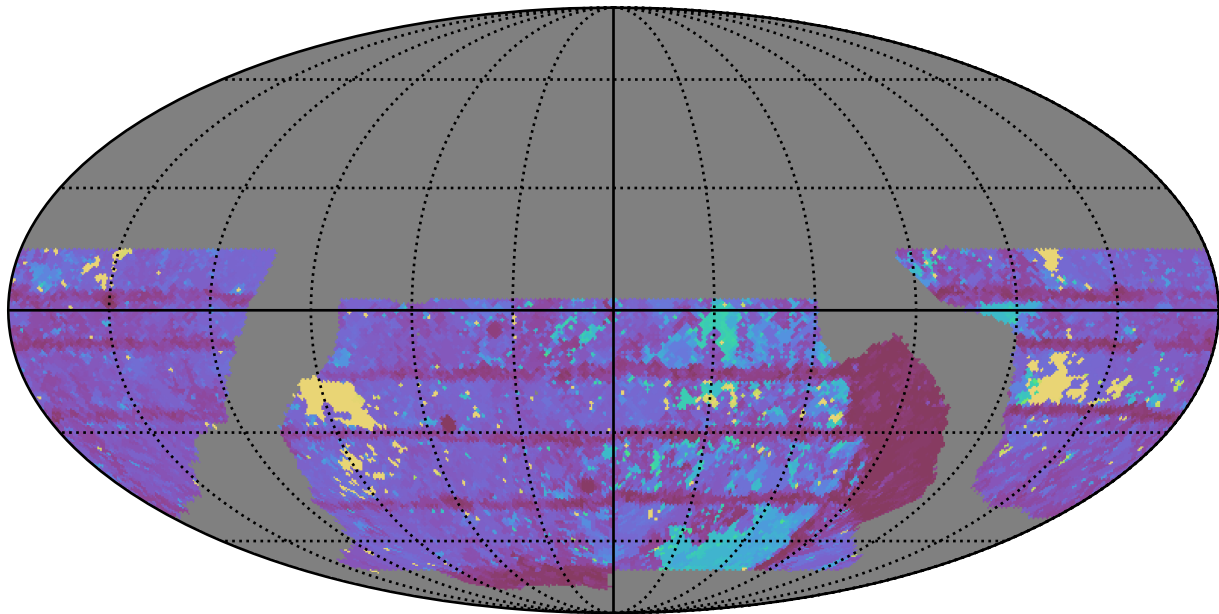
baseline_v2.0_10yrs WFD i band: Max Inter-Night Gap
