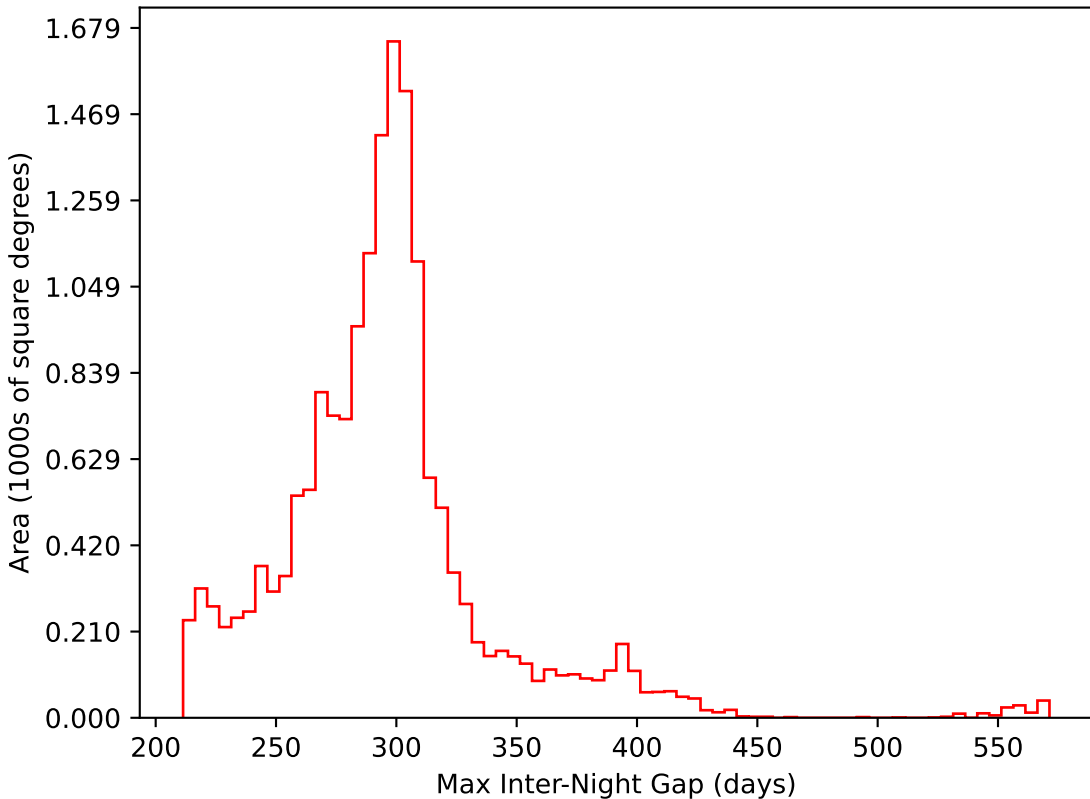
baseline_v2.0_10yrs WFD i band: Max Inter-Night Gap
