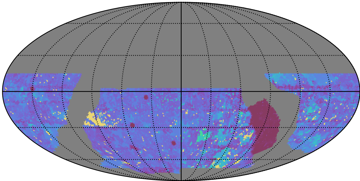
baseline_v2.0_10yrs WFD g band: Max Inter-Night Gap
