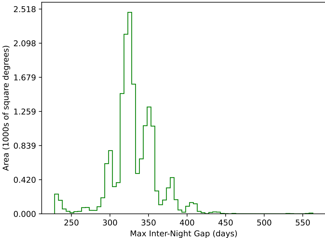
baseline_v2.0_10yrs WFD g band: Max Inter-Night Gap
