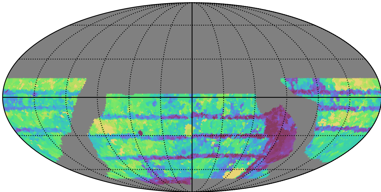
baseline_v2.0_10yrs WFD all bands: Max Inter-Night Gap
