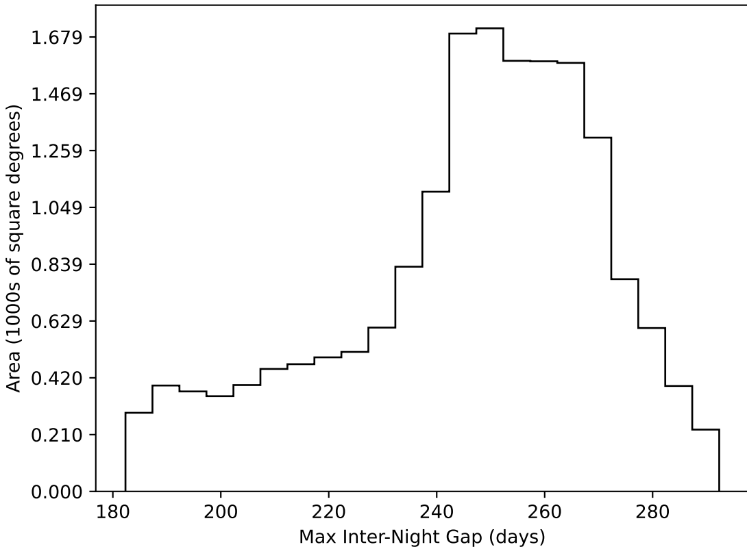
baseline_v2.0_10yrs WFD all bands: Max Inter-Night Gap
