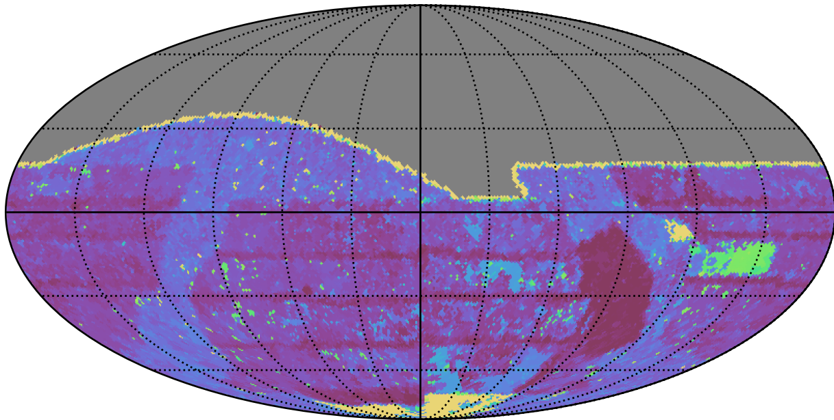
baseline_v2.0_10yrs All sky z band: Max Inter-Night Gap
