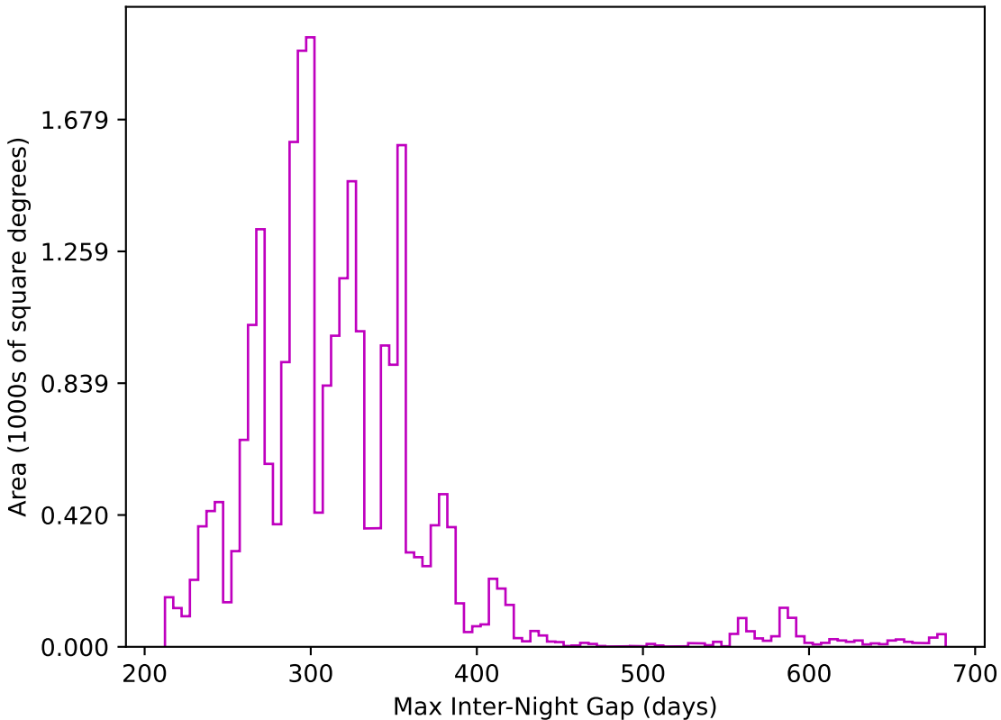
baseline_v2.0_10yrs All sky z band: Max Inter-Night Gap
