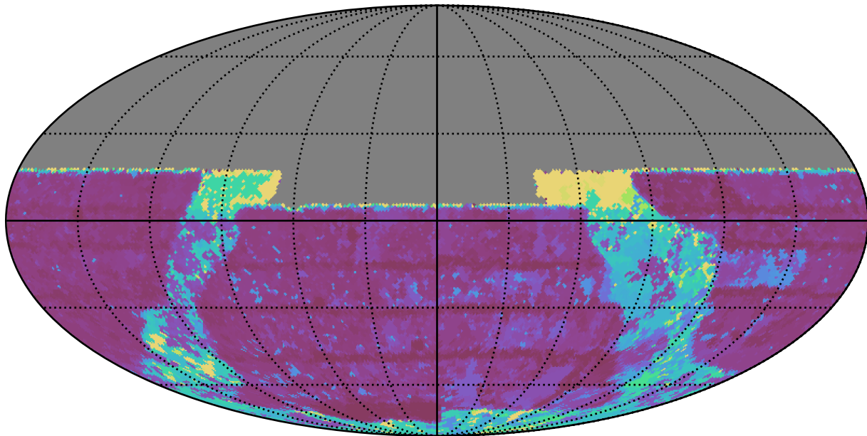
baseline_v2.0_10yrs All sky y band: Max Inter-Night Gap
