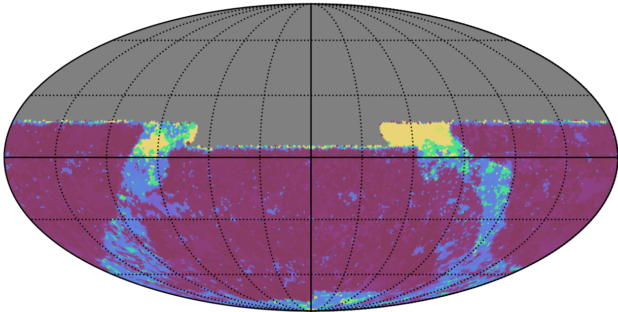
baseline_v2.0_10yrs All sky u band: Max Inter-Night Gap
