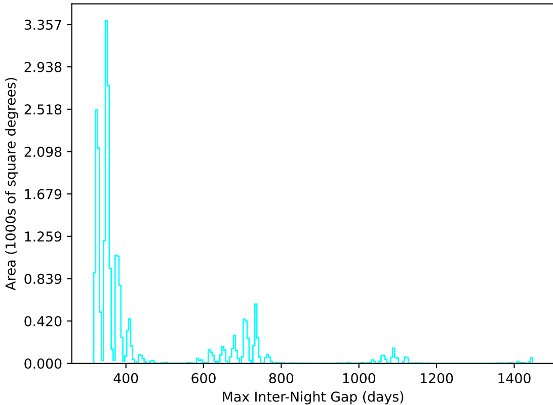
baseline_v2.0_10yrs All sky u band: Max Inter-Night Gap
