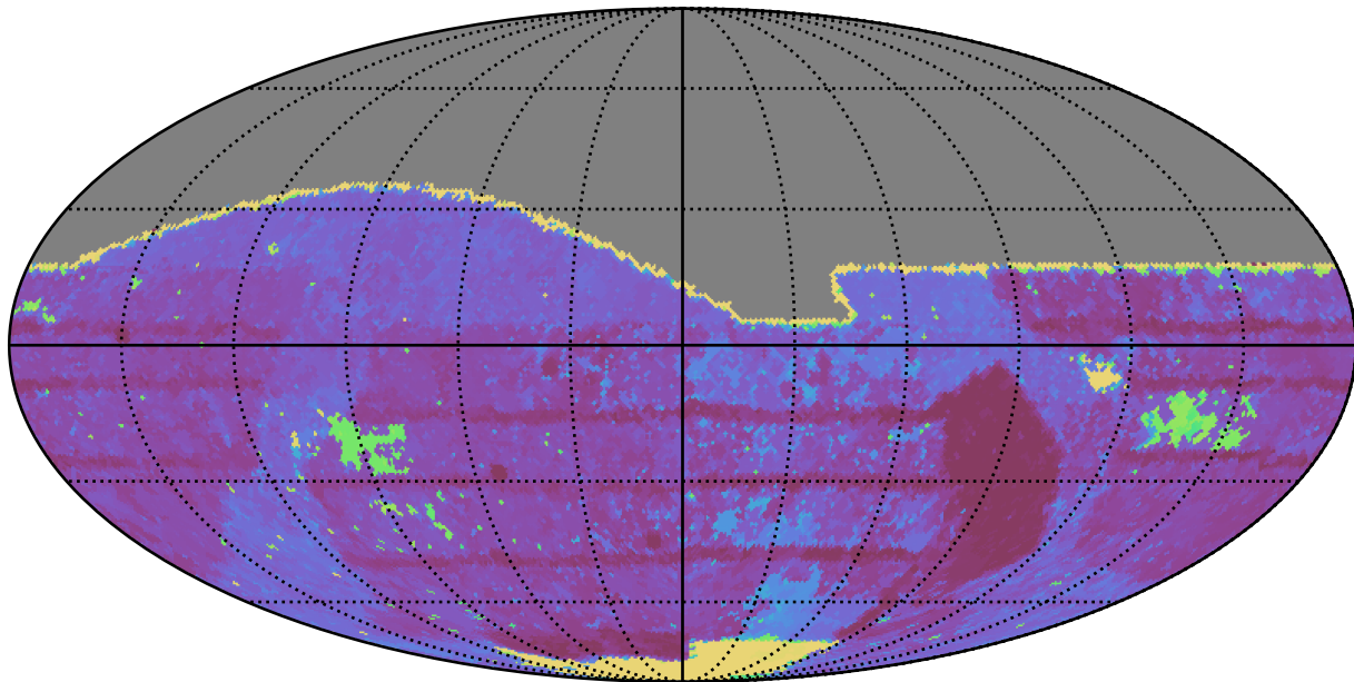
baseline_v2.0_10yrs All sky r band: Max Inter-Night Gap
