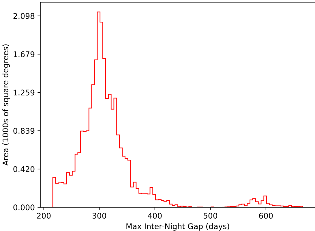
baseline_v2.0_10yrs All sky i band: Max Inter-Night Gap
