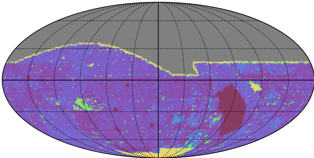
baseline_v2.0_10yrs All sky g band: Max Inter-Night Gap
